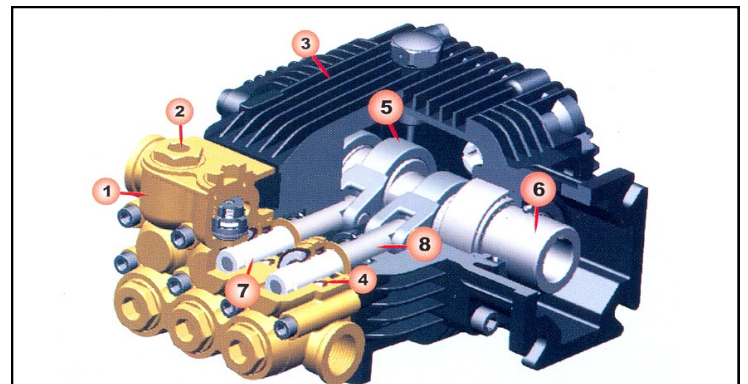
KleenMaster range of pressure washers features our Heavy-Duty DN range of pump heads. They come with 1) solid brass manifold, 2) Port plug with inner hex 3) anodized crankcase, 4) Super long life packing sleeves. 5) Oversized, one-piece connecting rod 6) Forged, precision grounded and hardened crankshaft. 7) Full ceramic plungers, stainless steel valves 8) Stainless steel plunger guide with heat treatment 9) Stainless steel valves for long life
