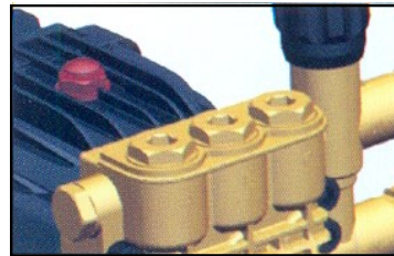
KleenMaster High Pressure cleaners features a heavy duty pump head with a pressure adjustable by-pass valve for long hours of continuous duty.
